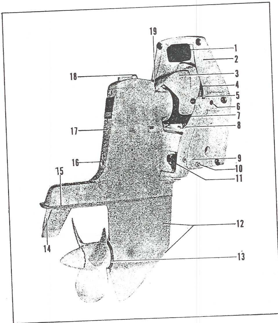
Fig. 1 Outboard Drive
